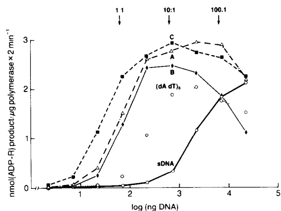
Fig.2. Effect of various concentrations of sDNA and octadeoxyribonucleotides on rates of polymer formation by poly(ADP-ribose) polymerase. \text{NAD}^+ concentration was 200 \mu\text{M} and 10 \mu\text{g} whole thymus histones were added per 0.10 ml incubation mixture.
